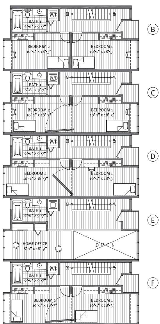
SECOND FLR. PLAN
