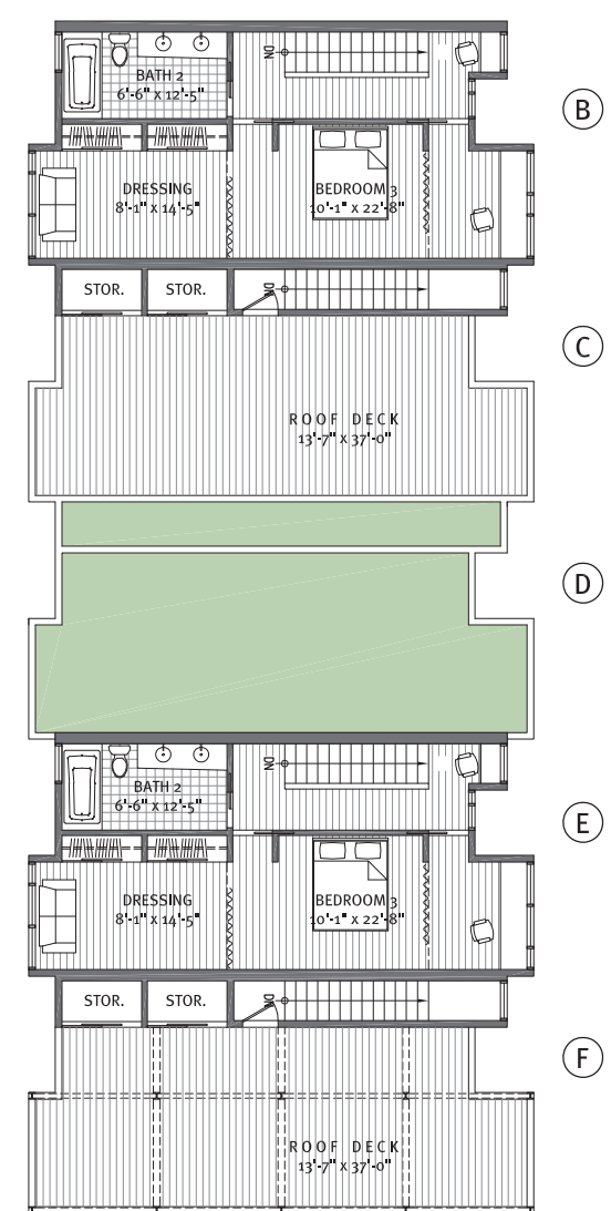
FOURTH FLR. PLAN
