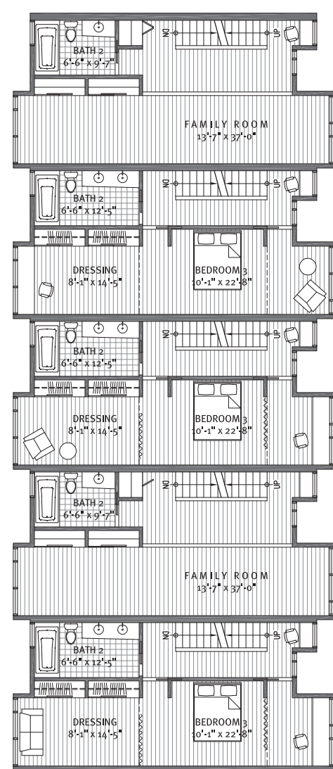
THIRD FLR. PLAN
